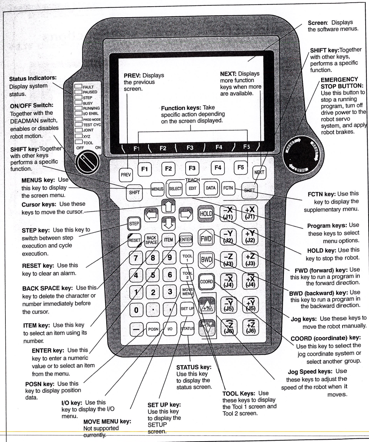
Figure 4-8 Teach Pendant
